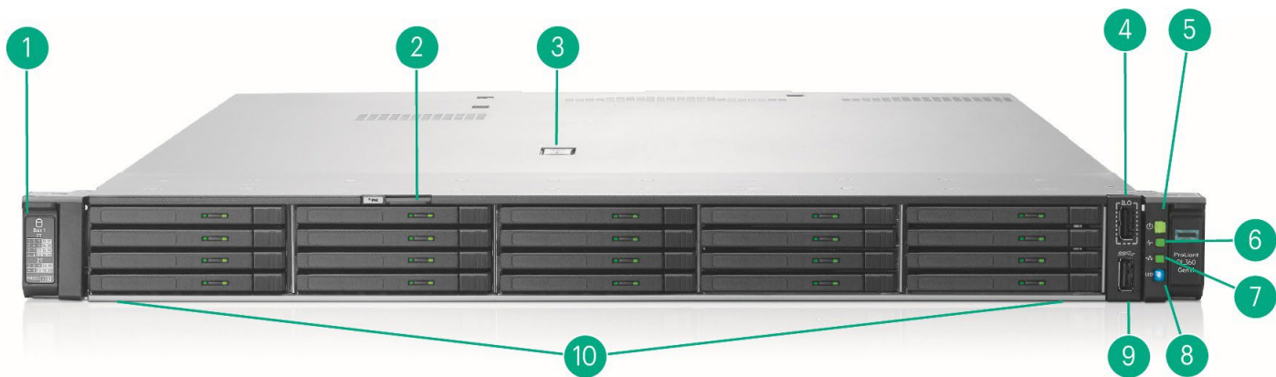
20 EDSFF Front View – 20 E3.s 1T NVMe drives shown
