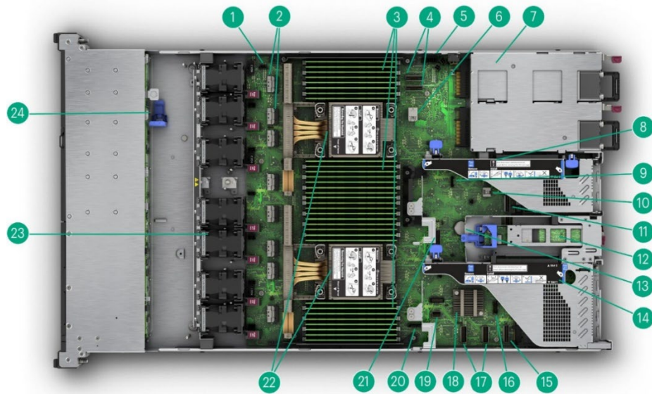
Internal View - Standard for all DL360 Gen11
